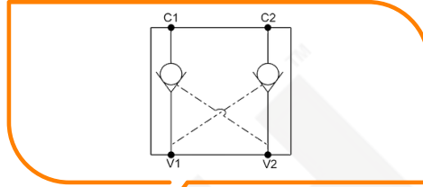
Hydraulic Circuit
