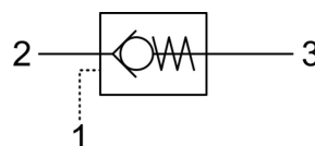
HYDRAULIC SYMBOL
